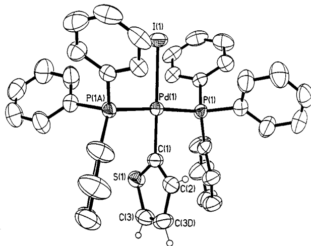
Fig. 3 An ORTEP 17 plot of the molecular structure of trans -[PdI(C 4 H 3 S-C)(PPh 3 ) 2 ] 2 (50% probability ellipsoids).
